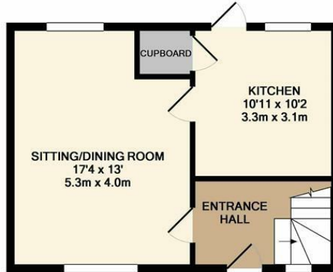
GROUND FLOOR APPROX. FLOOR AREA 402 SQ.FT. (37.4 SQ.M.)
